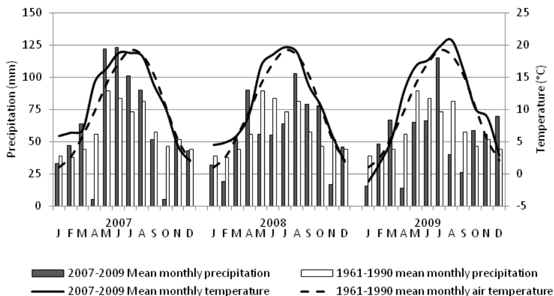
Figure 1. Climate data for Breisach Research Plot 2007 to 2009.
